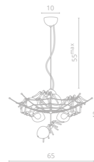
4 1308/02 SP-6 ∅65 | †43 | 55 max ⚡ 6x40W G9
