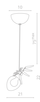
6 1308/02 SP-1 ∅21 | †22 | 75 max ⚡ 1x40W G9
